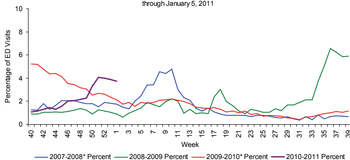
FIGURE 18: Percentage of Influenza-Like Illness from Emergency Department (ED) Chief Complaints, RDSTF Region 5 ESSENCE Participating Hospitals (N=49), Week 40, 2007 through January 5, 2011
