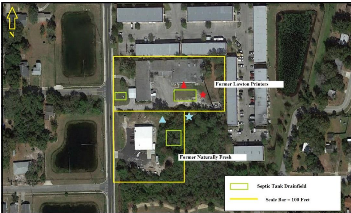
Figure 3: Anchor Road Solvent Site septic tank drain fields
