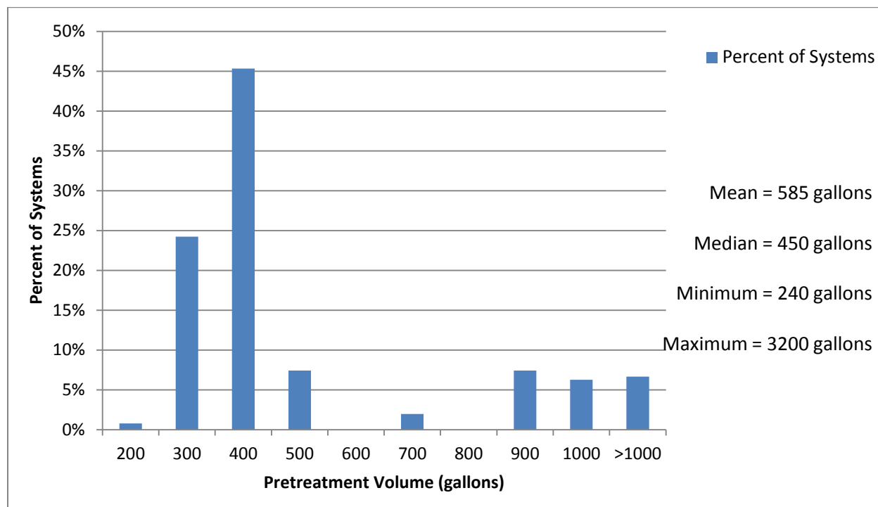
Figure 11. Distribution of Pretreatment Volumes in Gallons for Systems with This Information (n=256)
