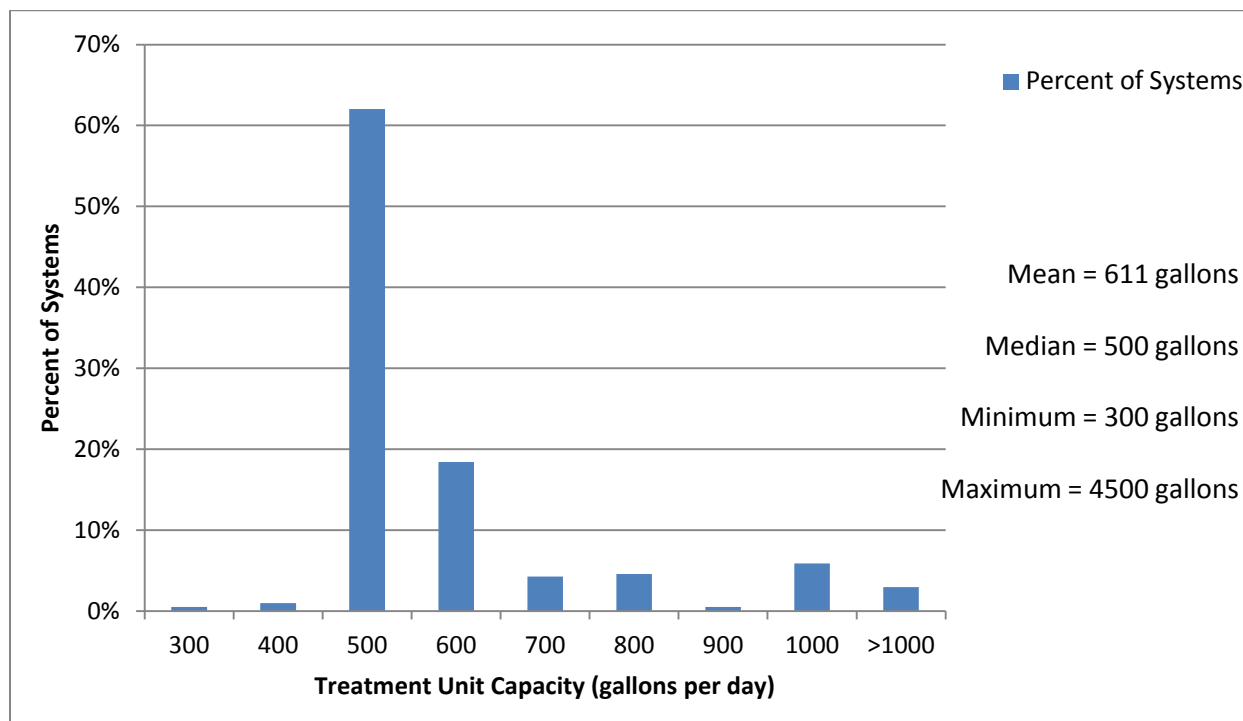
Figure 14. Distribution of the Hydraulic Capacity of the Treatment Unit in Gallons per Day (n=614)
