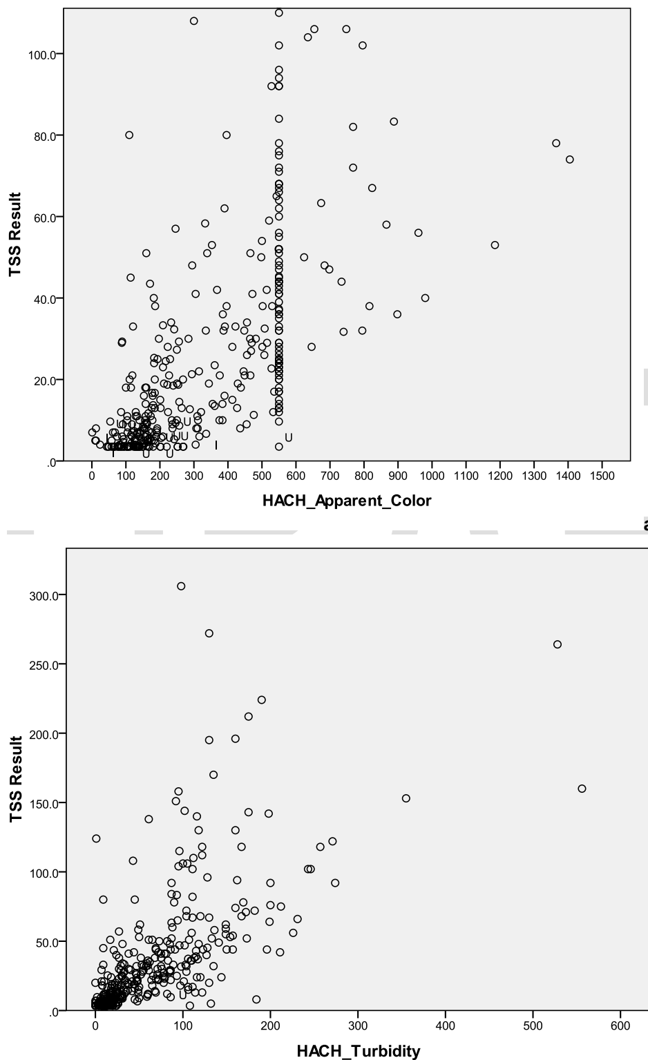
Figure 21. Concentrations of TSS Compared to Advanced OSTDS Field Instrument Measurements of a) Apparent Color and b) Turbidity. TSS-Scale is Not Fully Shown for Better Identification of Points
