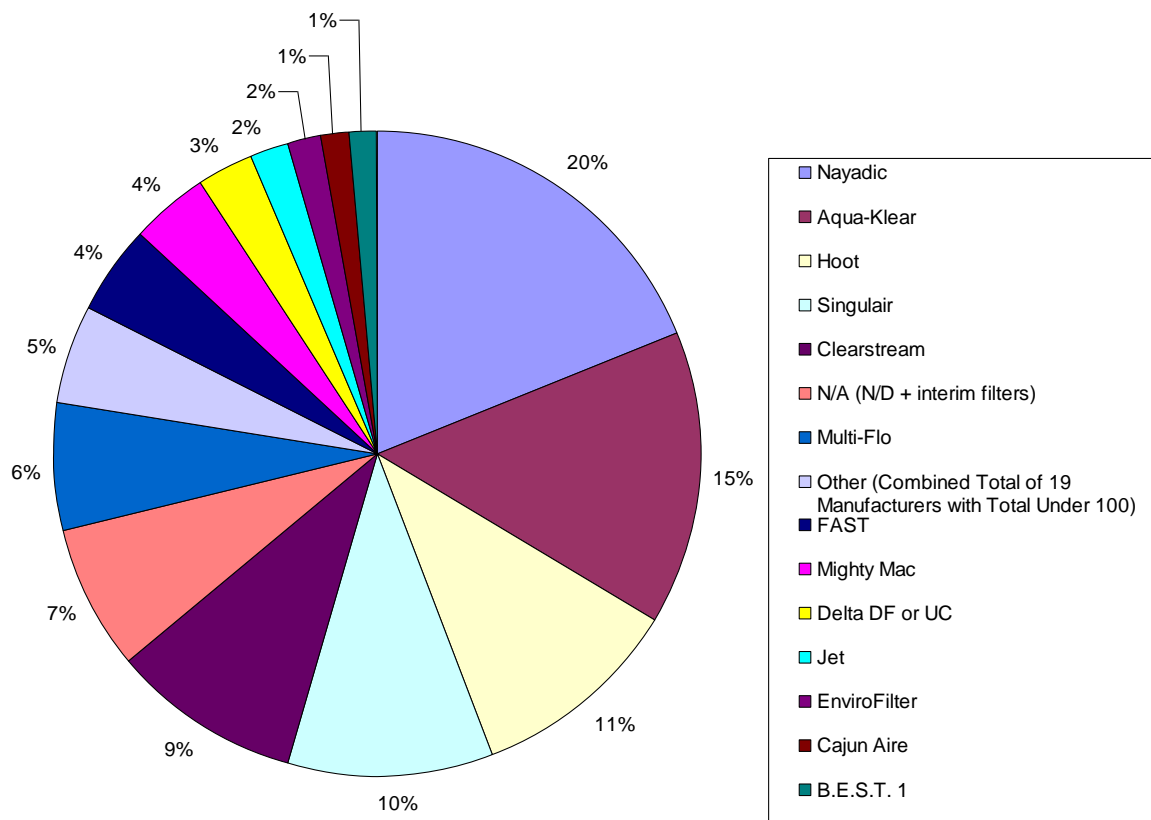
Figure 4. Product Technology for Systems with that Information (n=9,204)
