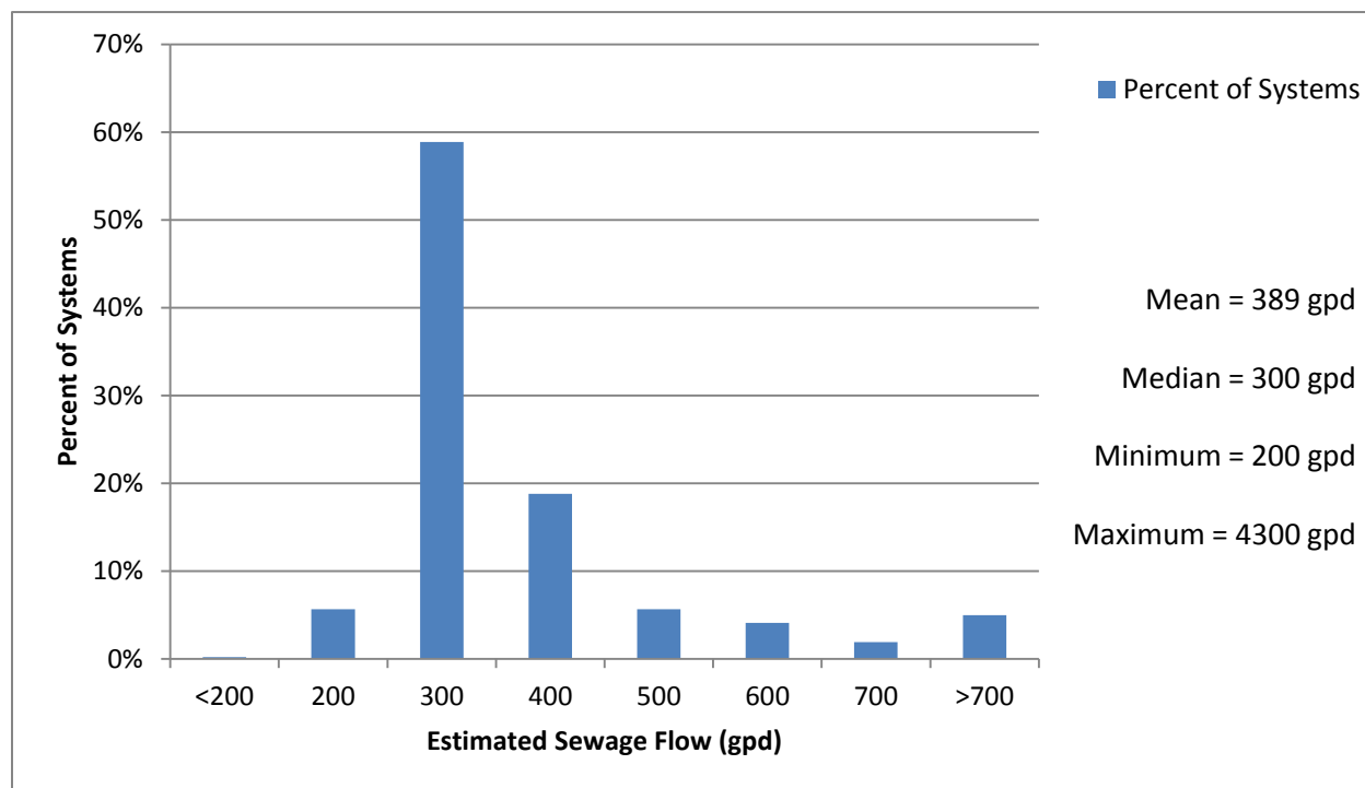
Figure 8. Distribution of Estimated Sewage Flow in Gallons per Day among Systems with a Documented Site Evaluation (n=586)
