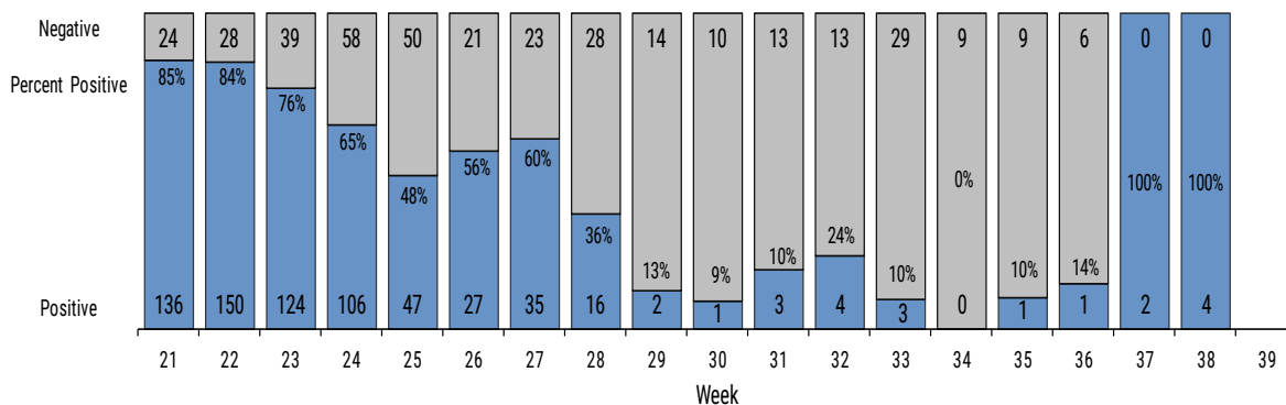
▲ The figure above shows the number of specimens tested for influenza at the Bureau of Public Health Laboratories (BPHL) by lab-event date, 1 week 21, 2022 to week 38, 2022. Specimens are organized by result and percent positivity of results was calculated by dividing positive results over total results.
