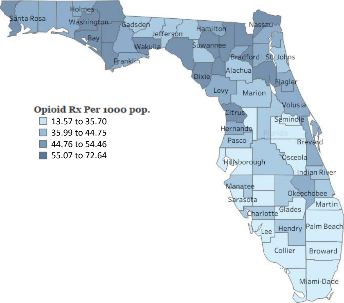
Age-Adjusted Opioid Prescription Rate by County, Florida Sep 2026
