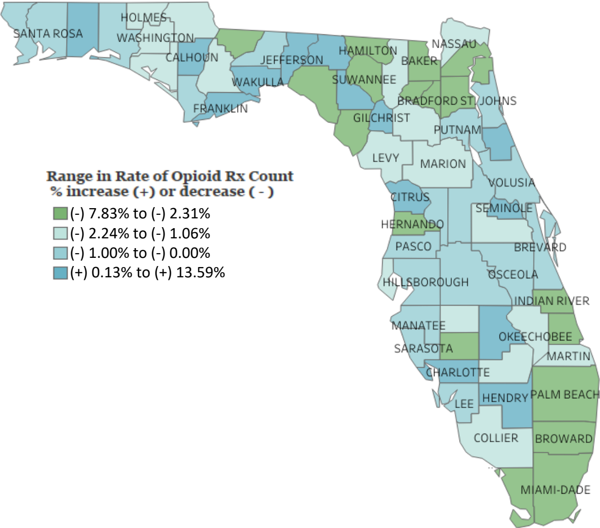
Percent Change in Opioid Prescription Count by County, Florida Jul 2026 - Sep 2026 vs Jul 2025 - Sep 2025
